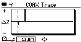
Figure 4. Run a coax TDR trace to see where large impedance changes are located.
